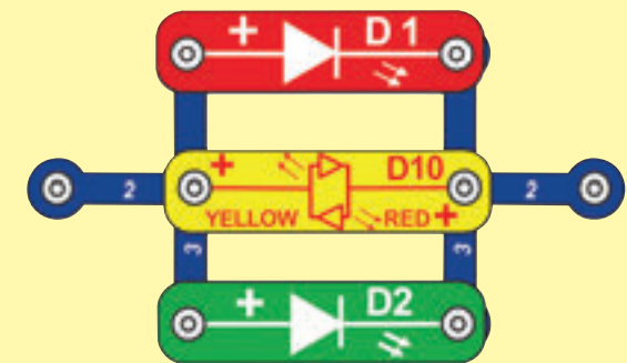
Parallel Circuit
